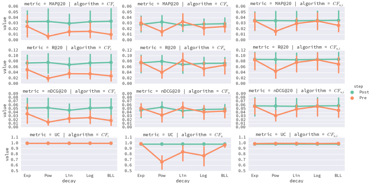
Figure 2: The figure summarises the results averaged over the five datasets in a 4 x 3 plot matrix. Rows are metrics (MAP@20, R@20, nDCG@20 and User Coverage), columns represent the methods ( CF_i , CF_u , CF_{u,i} ) and the x-axis of each plot shows the 5 decay-functions studied (Exponential, Power, Linear, Logistic, and BLL).
