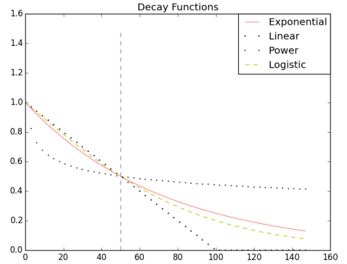
Figure 1: The figure compares the different decay functions at the step of parameter fitting. The x-axis represents temporal data (days since a bookmark was set) and the vertical blue dashed line is a median set on x=50 for representation purposes. BLL is not shown because its parameters are set based on literature.
