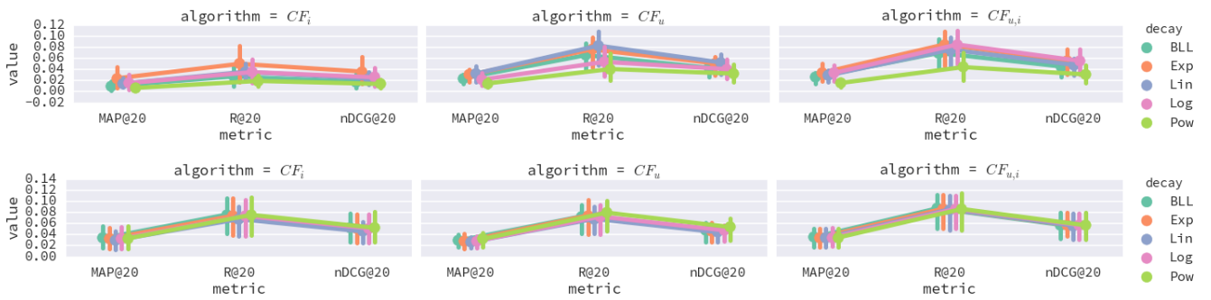
Figure 3: The effect (means over all datasets) of pre- (top row) and post-filtering (bottom row) with different decay functions and algorithms on the MAP@20, R@20 and nDCG@20 performance metric.
